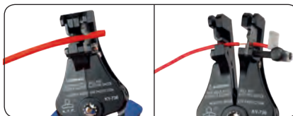
Attach the cable between the blades
