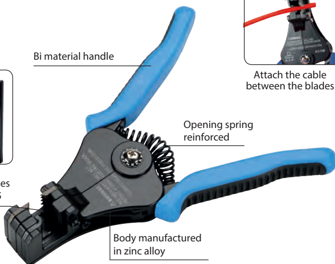
With length stop for repetitive work
